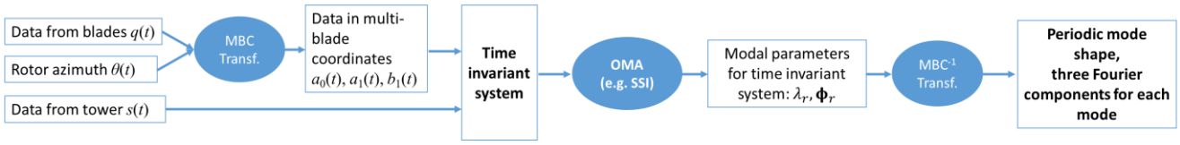
Fig. 1. Adaptation of MBC transformation to OMA
