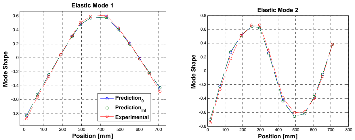
Figure 16. Predicted Mode Shapes
