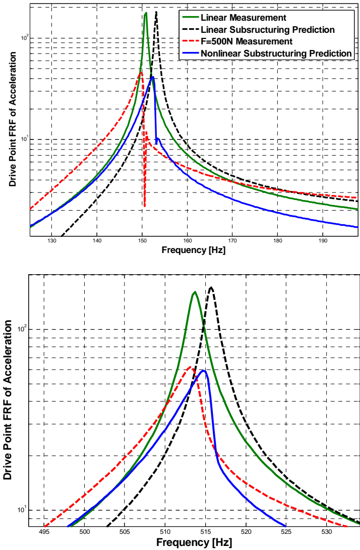
Figure 17. Frequency Domain Comparison: 1st Bending (Top) 2nd Bending (Bottom)
