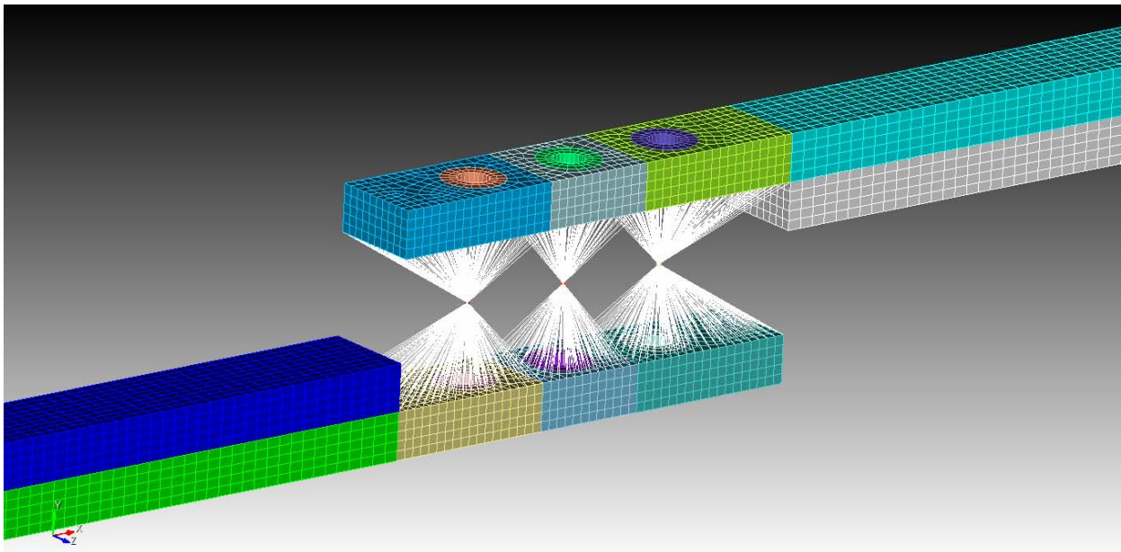
Figure 5. Finite Element Joint Surface Spider-Patch
