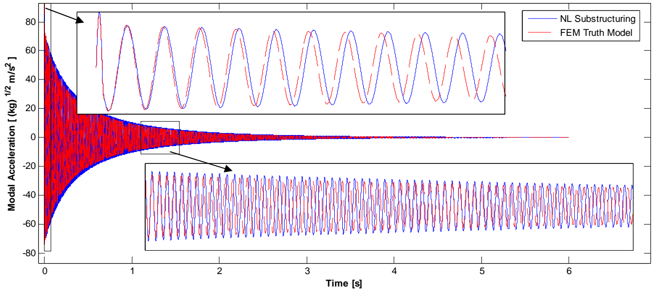
Figure 11. 1st Elastic mode: modal acceleration time history (Numerical Substructuring)
