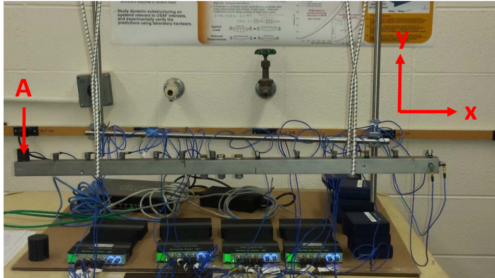
Figure 1. Brake-Reuss Beam Experimental Set-up
