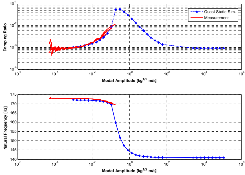
Figure 7. Quasi-Static results for amplitude dependent damping and frequency
