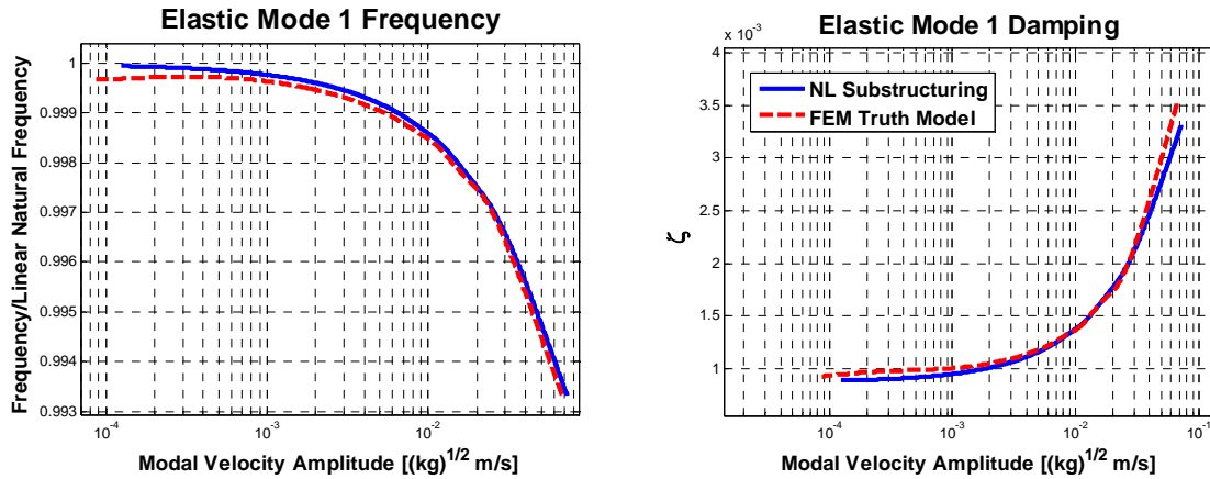
Figure 14. Amplitude dependent frequency and damping - 1 st elastic mode
