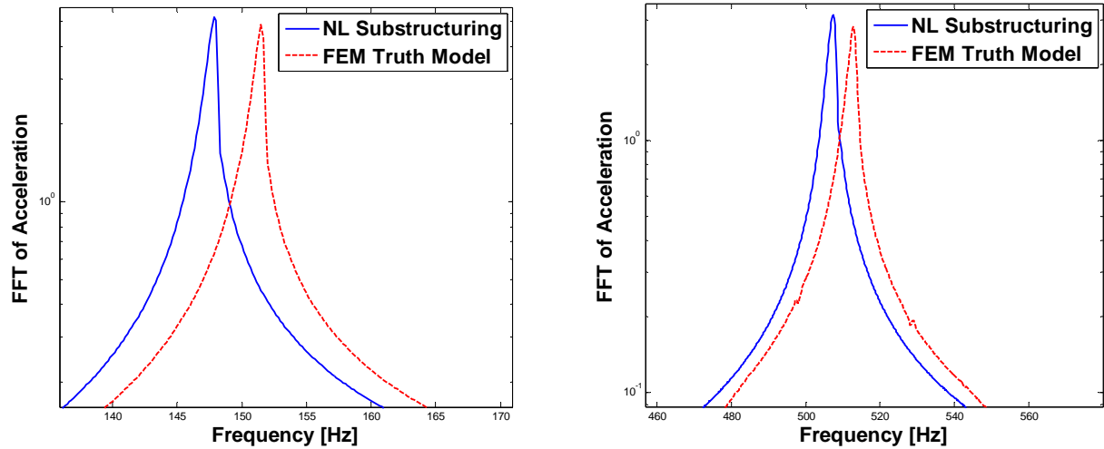
Figure 13. FFT of modal acceleration for 1 st (right) and 2 nd (left) elastic modes
