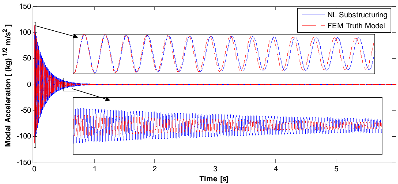
Figure 12. 2nd Elastic mode: modal acceleration time history (Numerical Substructuring)
