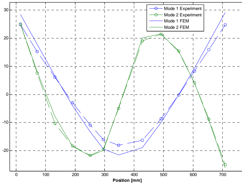
Figure 6. FEM and Experimental Mode Shapes
