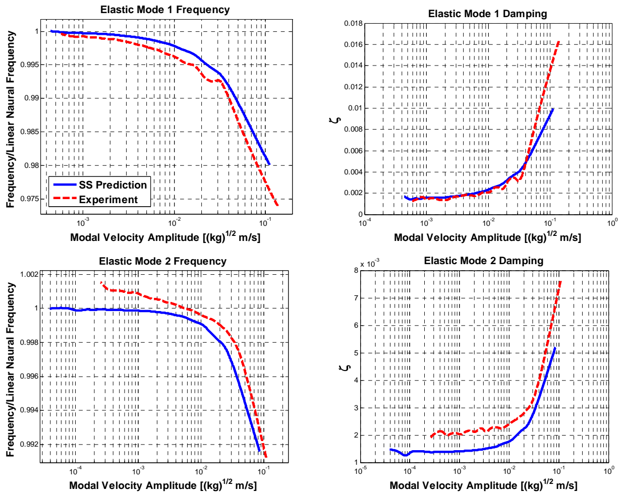
Figure 19. 1st and 2nd Elastic Mode: Amplitude Dependent Stiffness and Damping
