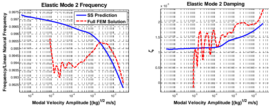
Figure 15. Amplitude dependent frequency and damping - 2 nd elastic mode
