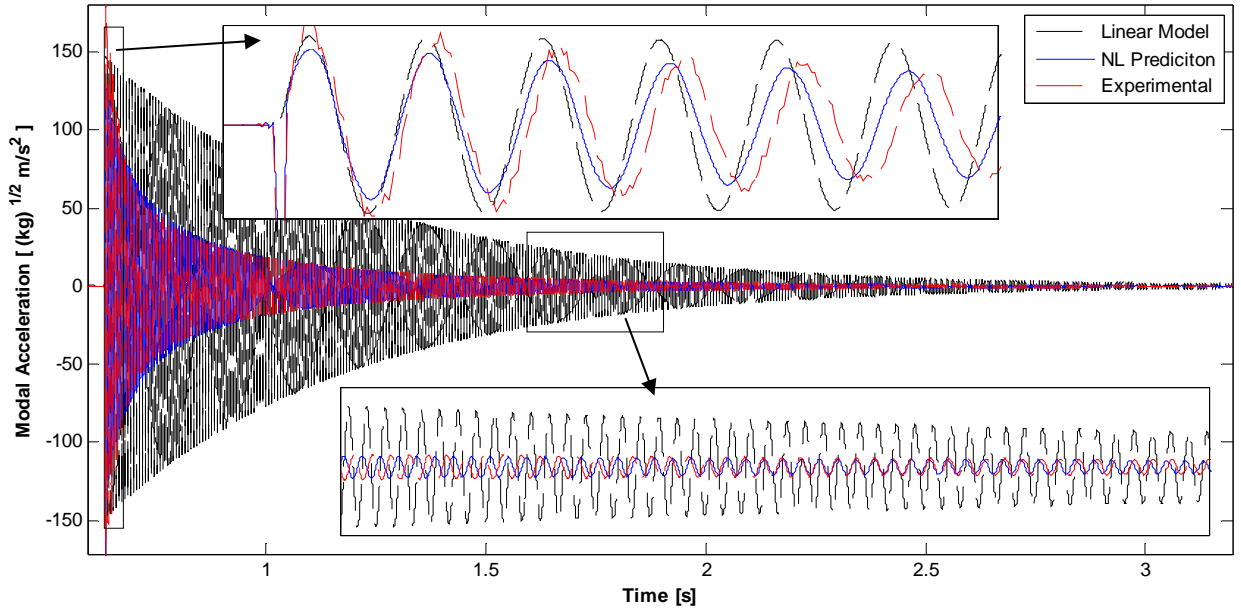
Figure 18. 1st Elastic mode: Modal acceleration time history
