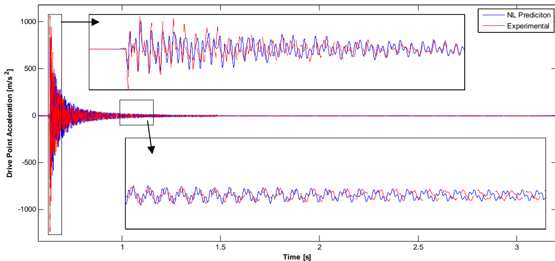
Figure 21. Drive point acceleration for 500N impulsive load
