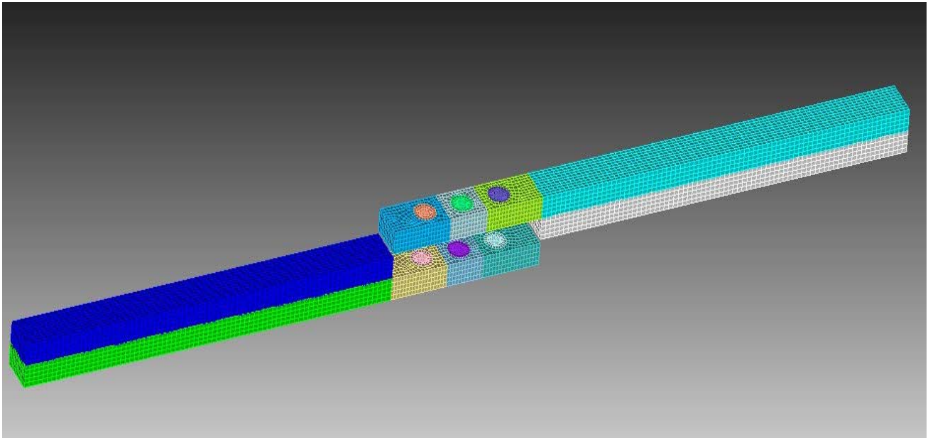
Figure 4. Finite element mesh for Brake-Reuss Beam substructure C
