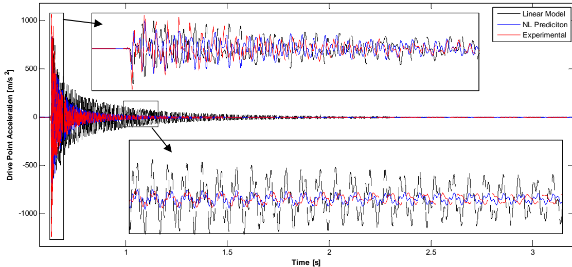
Figure 20. Drive point acceleration for 500N impulsive load with linear model
