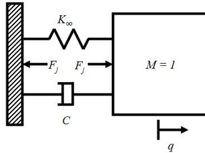
Figure 3. Schematic of SDOF model used for each modal degree of freedom
