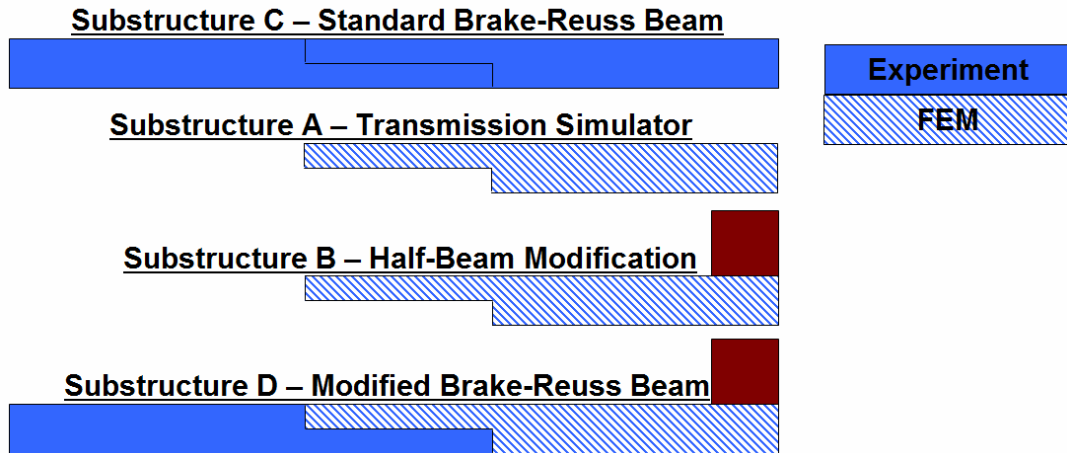
Figure 2. Substructure Overview
